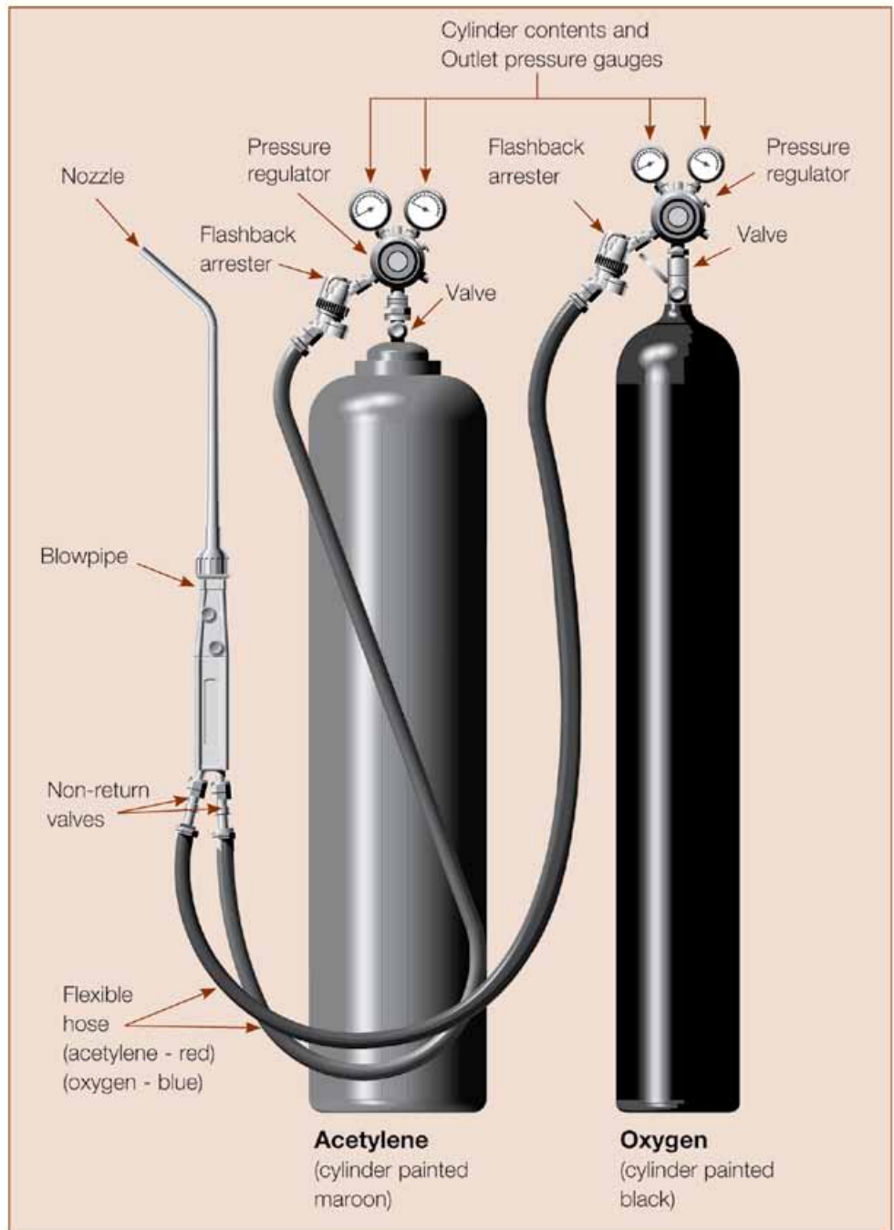
Figure 1 Typical equipment used in gas welding and allied processes
